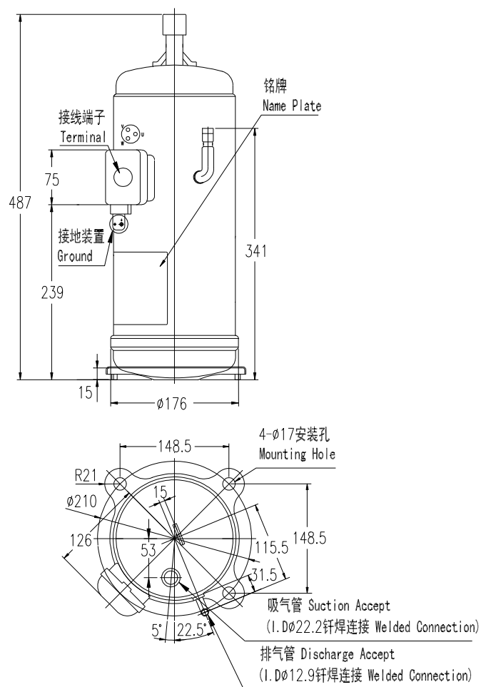
A-1 压缩机外形图 Dimension of Compressor (403DH-64C2)
