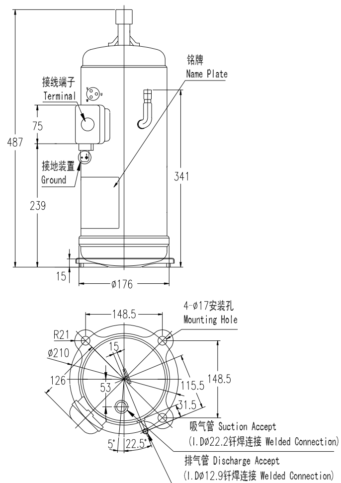
A-1 压缩机外形图 Dimension of Compressor (603DH-90C2)
